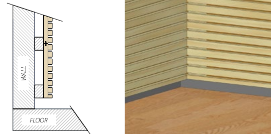
A detail of finishing the acoustic panel 50 mm above the floor
